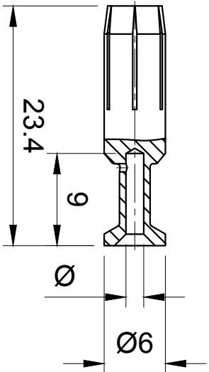
Female contact
