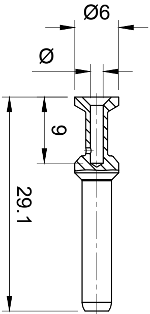
Male contact
