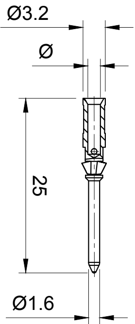
Male contact
