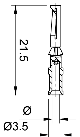
Female contact
