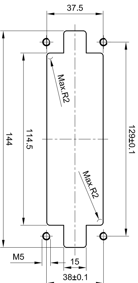
Panel cut out/面板开孔尺寸
