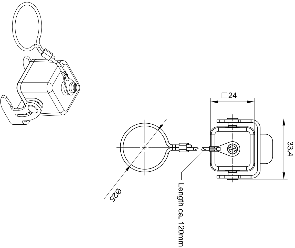
Metal cover for hoods with female insert
