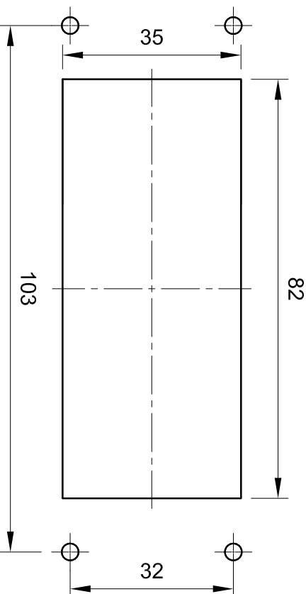
Panel cut out
