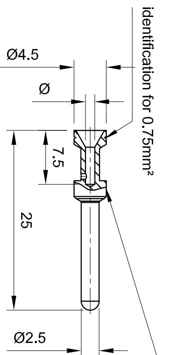
Male contact
