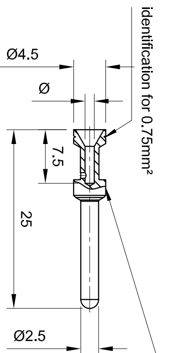
Male contact
