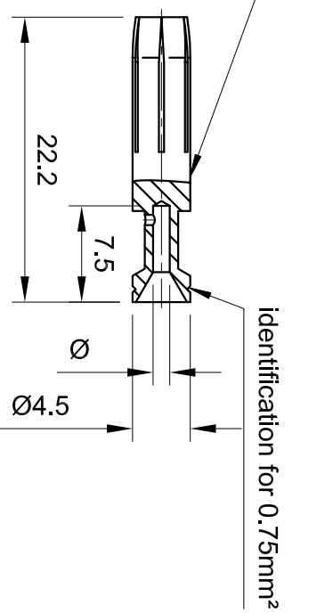
Female contact
