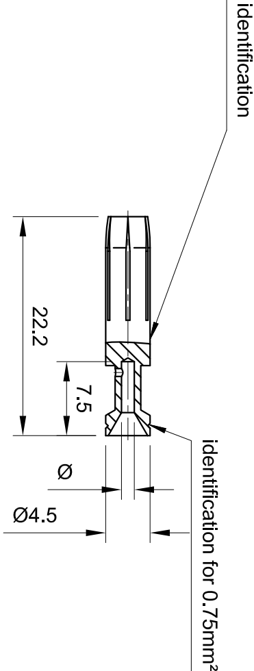
Female contact
